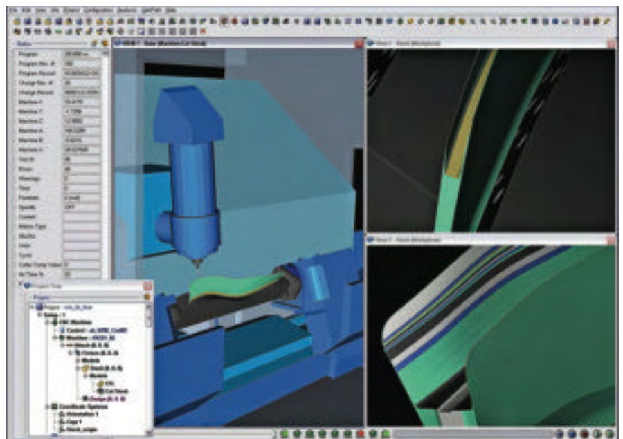
To prove that a 5-axis milling process could work for the GENx leading edges, every process element was first tested in the Vericut virtual environment.
